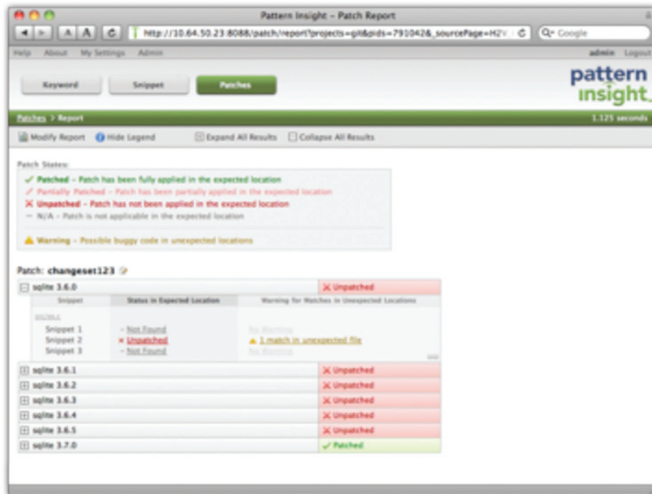
Figure 1: Code Assurance Report
